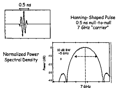
Fig. 3. Example of a narrow ultrawideband pulse occupying \sim 5 GHz of spectrum.
